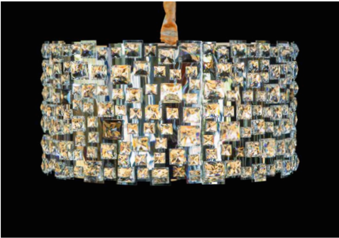
FACETS 6 LIGHT CHANDELIER LT-CH964-6CLR Dimensions: 11 3/4" h x 13 3/4" dia Net Weight: 18 lbs Number of Lights: 6 Light Bulb Type: E12 Chain Included: 3 ft
